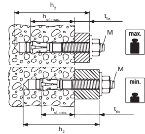
Bolt anchor FAZ II GS (with large washer) / FAZ II HBS (washer compliant to timber construction standard DIN 1052)
