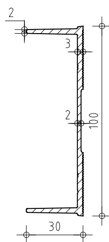
C-channel 100x30
