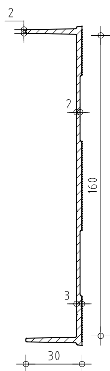
C-channel 170x30
