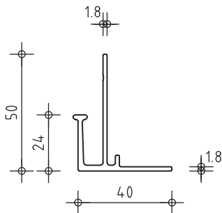
ATK 106 main section Art. 663003
