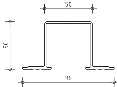
ATK 106 hat section Art. 663004
