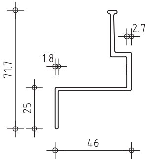
ATK 106 Z section Art. 663001
