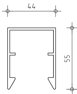
U-support section Art. 68305
