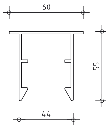
PI-section-60 Art. 68806
