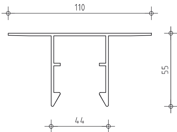
PI-section-110 Art. 68807
