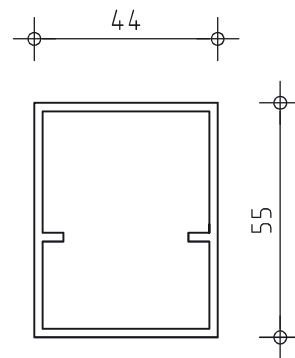
Box section Art. 66000
